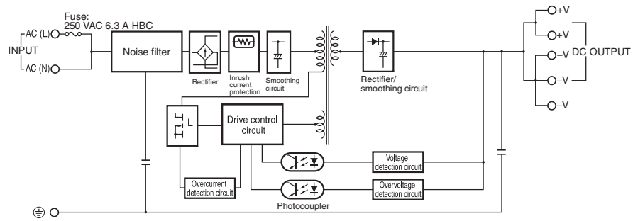
S8VK-C06024 (60W)
