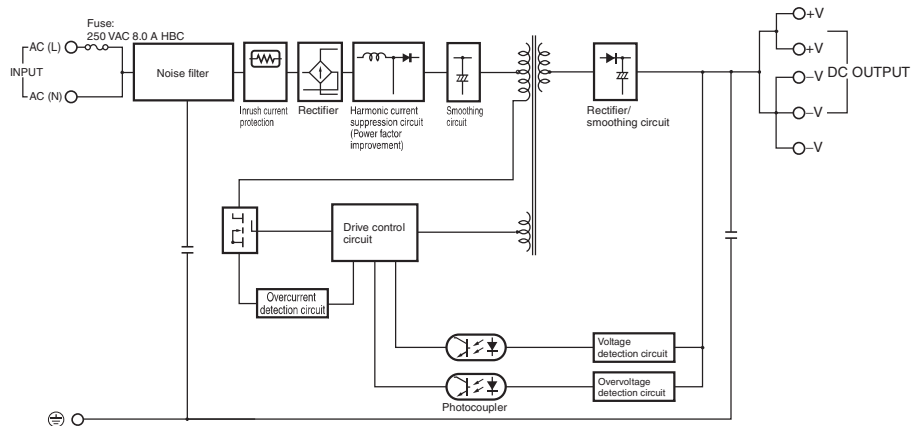
S8VK-C24024 (240W)
